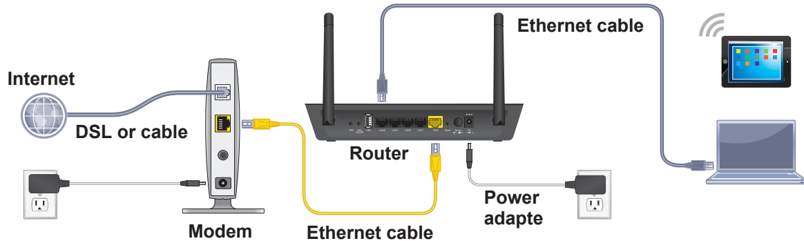
Figure 3. Router cabling
