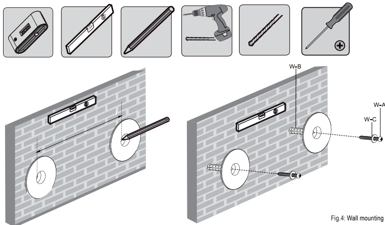
Fig.4: Wall mounting
