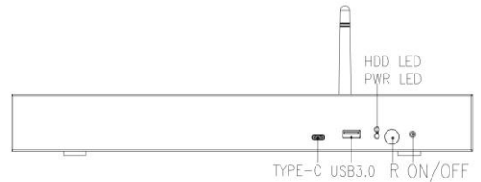
Front Panel External I/O
