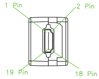
HDMI Female (Out Put)
