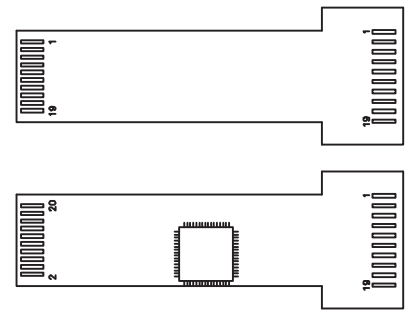
PCB Pin Assignment
