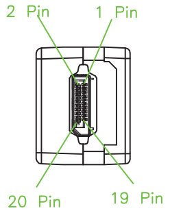
Display Port Male (Input)
