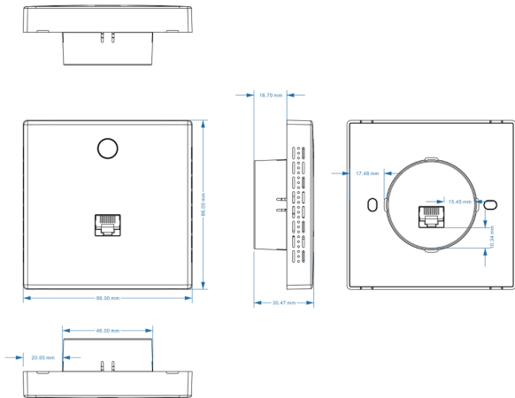
Product Dimensioning Diagram :
