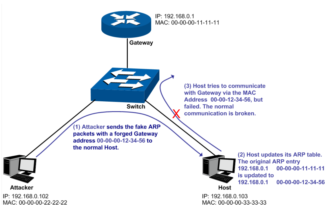
Figure 13-10 ARP Attack - Imitating Gateway
