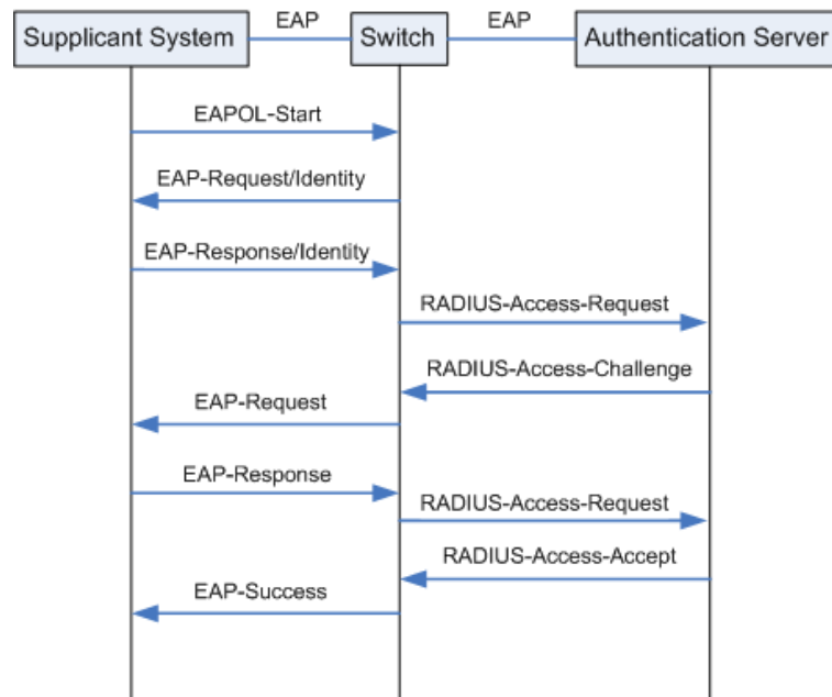
Figure 13-19 EAP-MD5 Authentication Procedure
