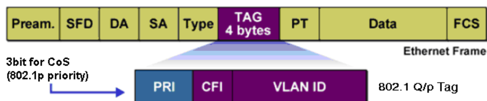
Figure 10-2 802.1Q frame
