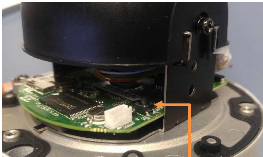
Reset Button
