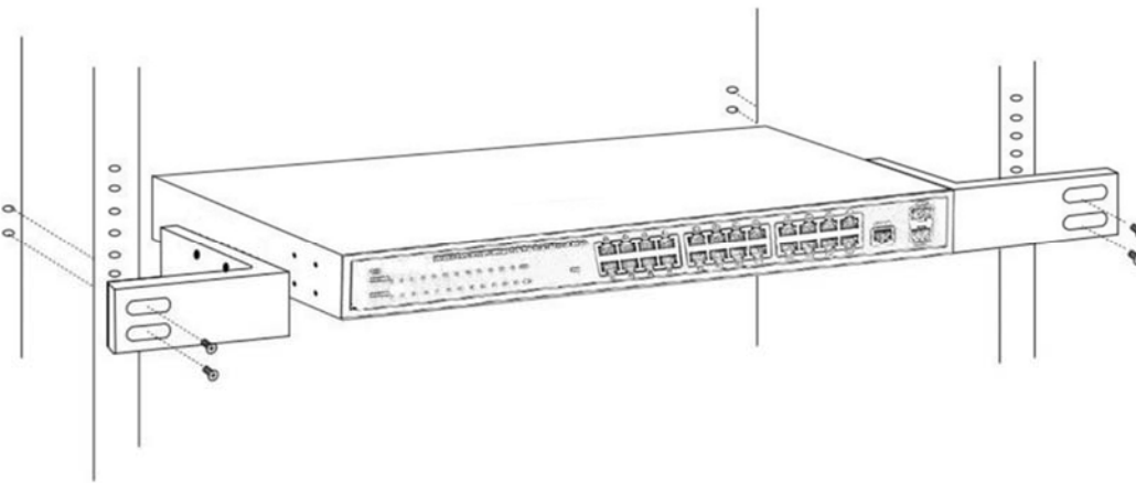
Figure 6 - Rack Installation
